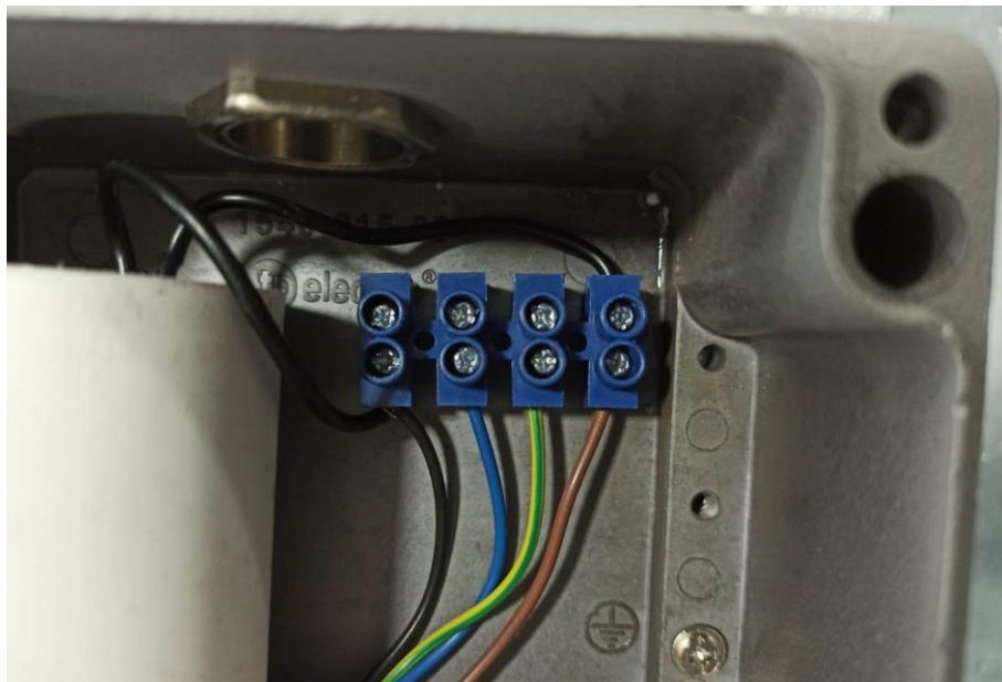
Photo 10. Terminal
