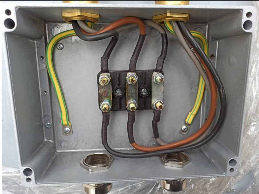
Photo 7. Connection Box
