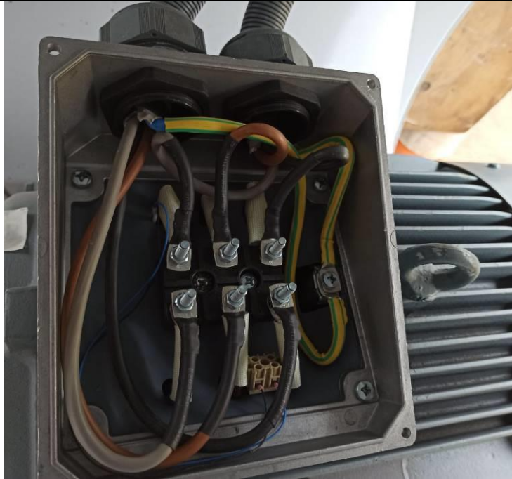
Photo 9. Motor Connection
