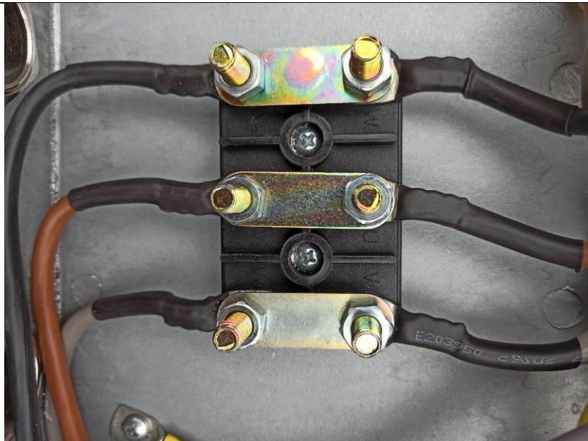
Photo 10. Terminal
